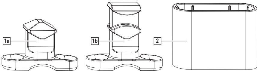
Fig. 7.1: [1a] Locking pin without night ventilation; [1b] Locking pin with night ventilation; [2] Packer
