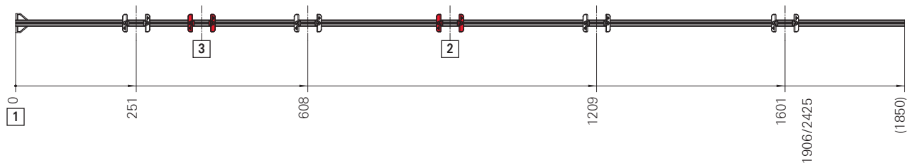
Fig. 9.3: [1] Roller track stop; [2] Adapter position for locking pin 1906; [3] Adapter position for locking pin 2425
